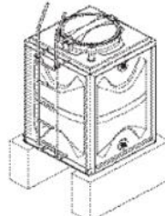
1 \times 1 \times 1.5 = 1.5\text{m}^3 3.3 x 3.3 x 4.9' = 396 USG
